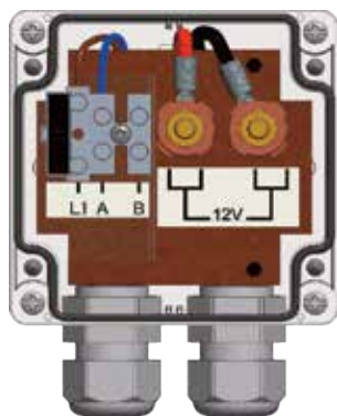
STANDARD TERMINAL ENCLOSURE 80VA TO 750VA
