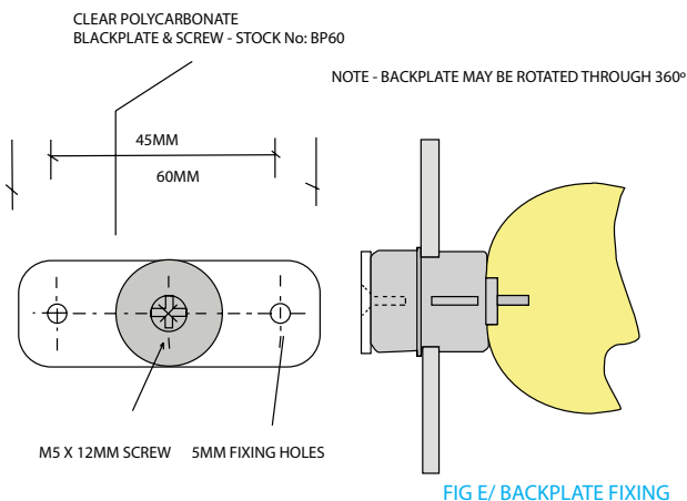
FIG E/ BACKPLATE FIXING
